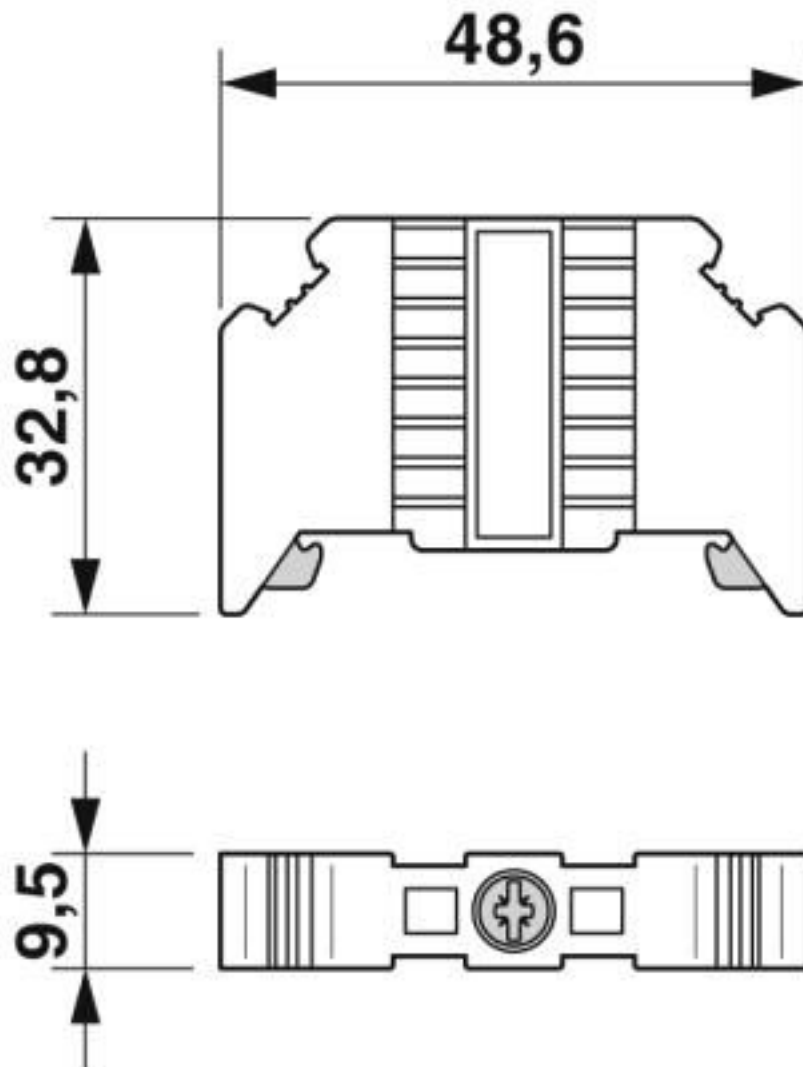
Dimensional drawing
